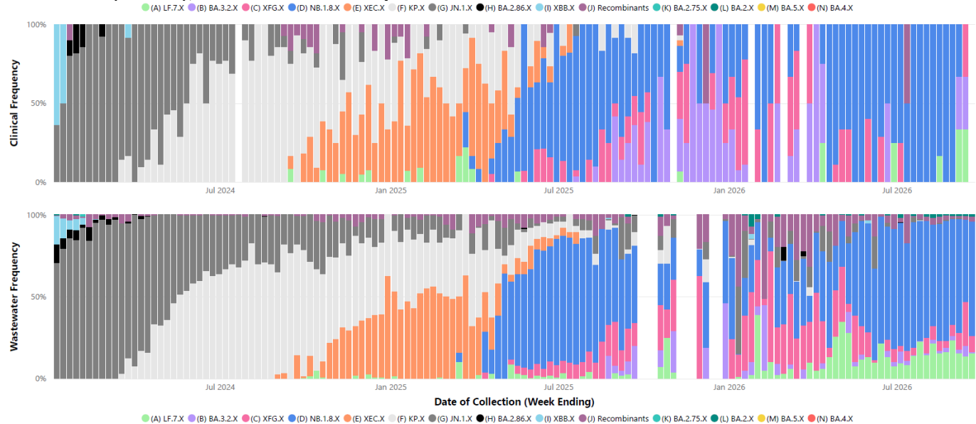
Figure 18. Distribution of SARS-CoV-2 variants in clinical samples (top) and metropolitan wastewater catchments (bottom), 01 Jan 2024 to 20 Sep 2026
